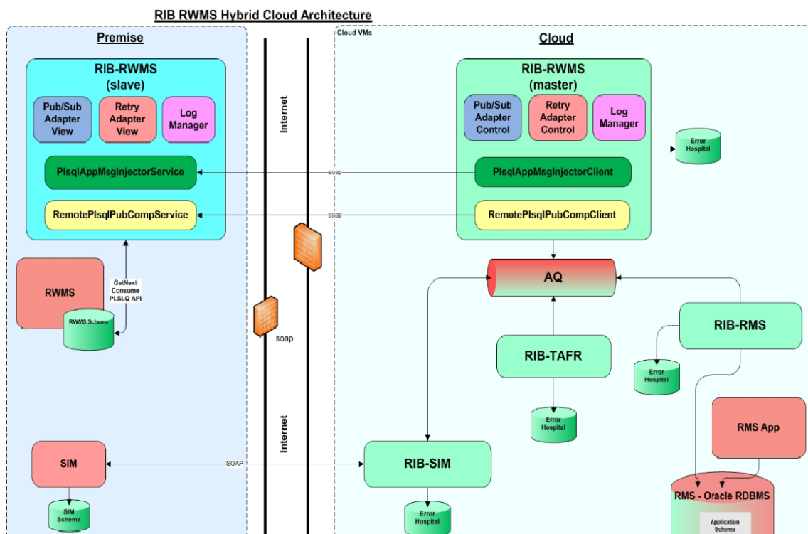
Figure 7-2 RIB-RWMS Hybrid Cloud Architecture
